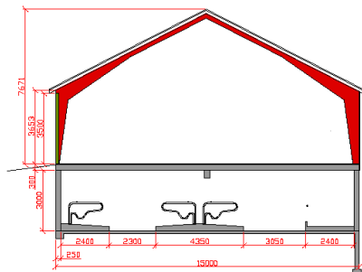
SNITT A - A (1:100):
